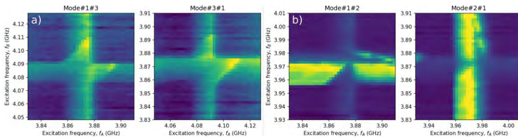
Figure 1: Delayed two-tone parametric spectroscopy maps with nonlinear frequency shifts (a) and non-commutativity (b).
