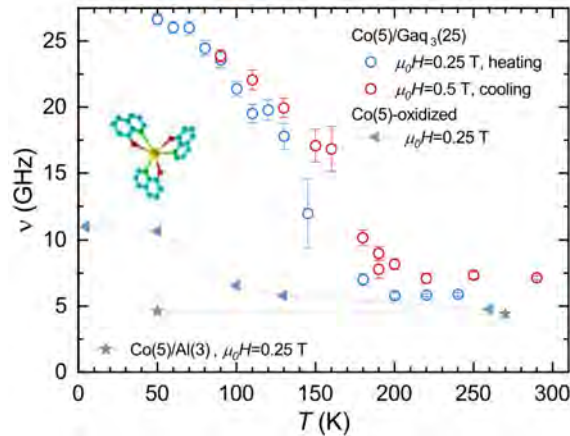
Figure 1: The spin-wave frequency as a function of temperature at a constant external magnetic field in the Co(5 nm)Ga 3 (25 nm) sample compared to the reference Co(5 nm)/Al(3 nm) sample and oxidized Co(5 nm) film.
