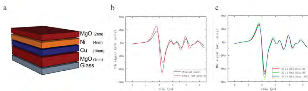
Figure 1: (a) Cu/Ni multilayers deposited on a glass substrate. (b) Enhancement of terahertz emission in the Cu/Ni sample upon irradiation. (c) Comparison of terahertz signals under different irradiation conditions.
