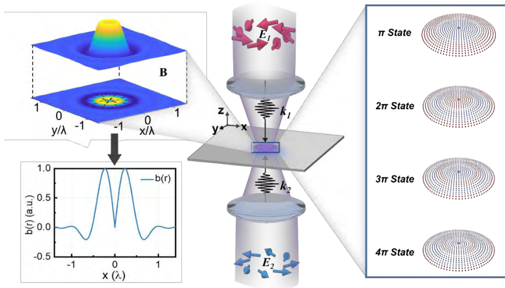
Figure 1: Creation of topological spin textures by a radially polarized magnetic field induced by the inverse Faraday effect. Two cylindrical vector beams with electric field \mathbf{E}_1 and \mathbf{E}_2 are tightly focused on the sample. Under different amplitude of the induced field, four stable topological spin textures can be created (the right inset).
