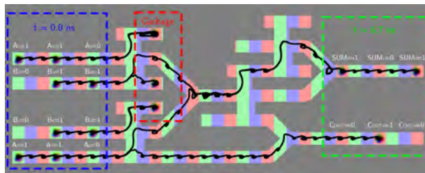
Figure 2. Micromagnetic simulation of pipelined full adder. Skyrmions are pipelined into the full adder from the left, encoding inputs ( A_0=0, B_0=1; A_0=0, B_0=1; A_1=1, B_2=1; A_3=1, B_3=0 ). Black lines represent their trajectories, and skyrmions are propagated according to the respective VCMA regions (light red/green/blue) using the VCMA waveform shown in Fig. 1(c). At t=0 ns (blue), the skyrmions are initialized and propagated rightward to the correct logical outputs at t=8.7 ns (green).
