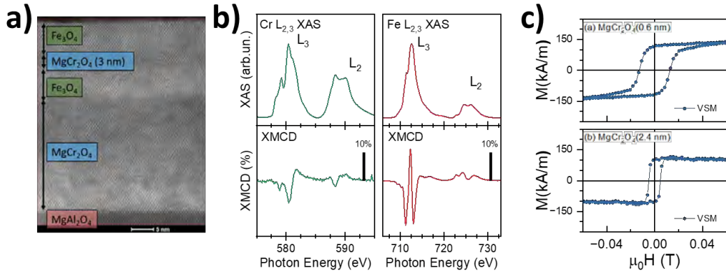
Figure 1: STEM image of one of the investigated heterostructure (a) and corresponding XAS and XMCD spectra around the Fe L_{2,3} and Cr L_{2,3} edges (b). (c) Hysteresis loops measured by VSM for two different \text{MgCr}_2\text{O}_4 spacer thicknesses.
