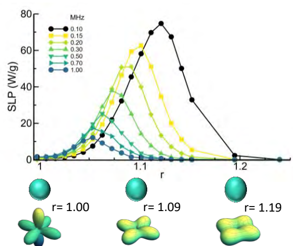
Figure 1: Specific loss power dependence on the aspect ratio ( r ) of magnetite NP of size D= 25 nm at different frequencies and ac field values complying with the Brezovich criterion.
