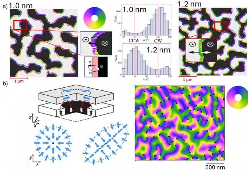
Figure 1: SEMPA results of dipole - iDMI competing systems (a) extracting the chiral nature (CW = clockwise, CCW = counter clock wise) of domain walls as a function of top ferromagnetic layer thickness (b) merons and anti-merons (black dots) as detected using SEMPA on a 2.4 nm thick Co top layer.
