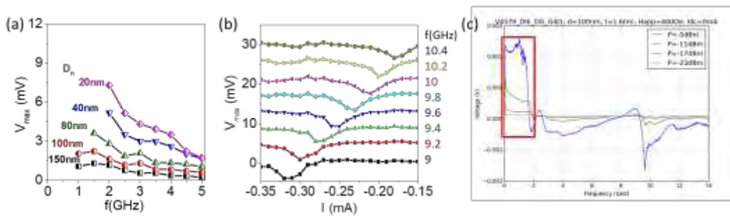
Figure 1: (a) Maximum rectified DC voltage vs. frequency for pMTJs of different diameters and a FL thickness t_{FL} = 1.8 nm. (b) Example of frequency tuning with DC bias current. (c) Broadband detection for a pMTJ device of t_{FL}=1.6 nm.
