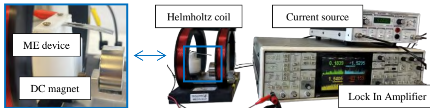
Figure 1: ME measurement set-up.
