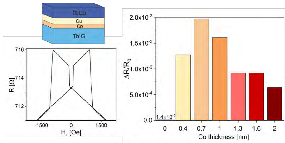
Figure 1: Left panel: Schematic of the TbIG/Co/Cu/TbCo spin-valve structure and resistance (R) as a function of out-of-plane field ( H_z ) for TbIG/Co (0.7nm)/Cu/TbCo. Right: Amplitude of the magnetoresistance ( \Delta R/R_0 ) for different thicknesses of Co insertion layer.
