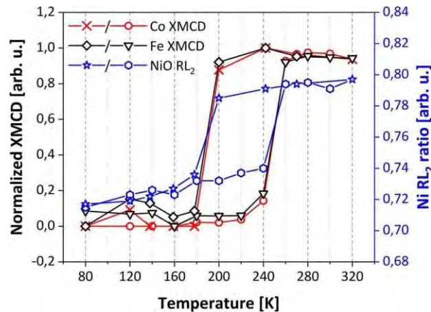
Figure 1: Temperature dependence of XMCD (black and red for Fe and Co respectively) and Ni XMLD (blue) in Co(10 Å)/NiO(40 Å)/Fe(104 Å) trilayer. Thermal hysteresis of the spin reorientation in Fe is mimicked by NiO and Co layers.
