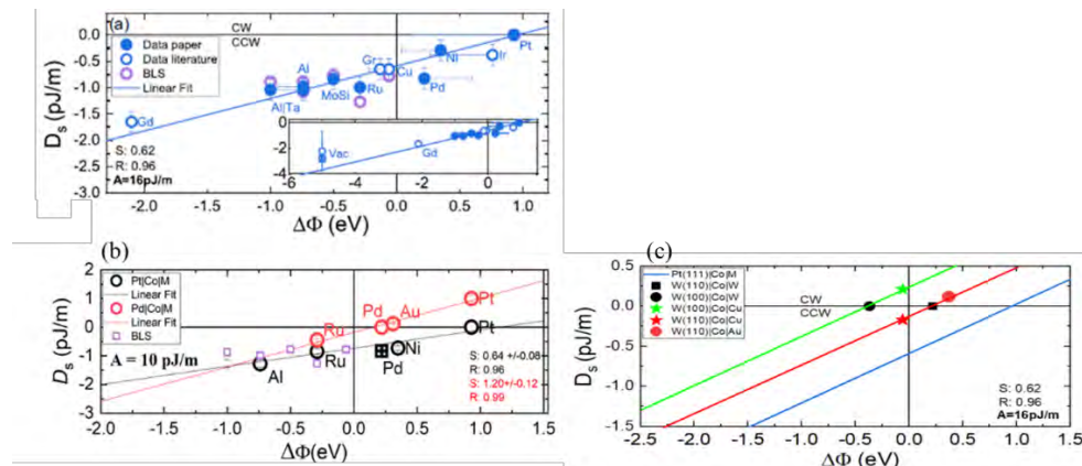
Figure 1 (a) D_s vs \Delta\phi of Pt|Co|M trilayers (b) D_s vs \Delta\phi of Pt|Co|M and Pd|Co|M multilayers with n=3 to 6 . (c) D_s vs \Delta\phi of W|Co|M with W 100 (green) and 110 (red)
