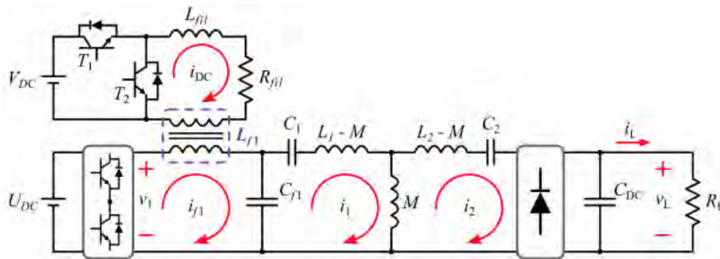
Figure 1: Scheme of the LCC-S compensated IWPT system with magnetic control, implemented through the controlled variable inductor L_{fi1} , supplied on the auxiliary winding with a synchronous DC-DC buck converter.
