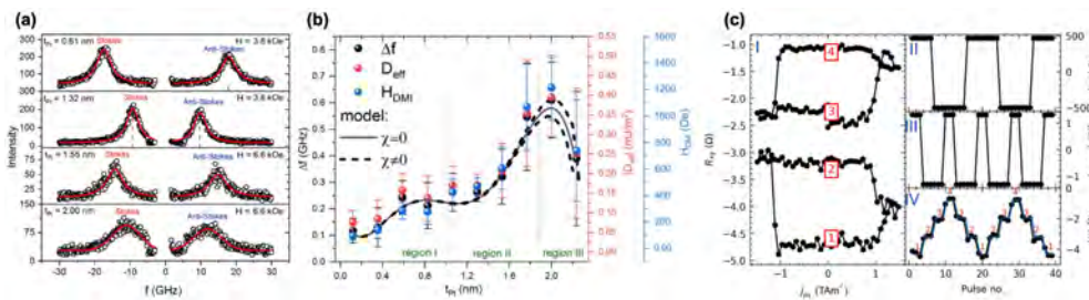
Figure 1. (a) BLS spectra of Stokes and anti-Stokes peaks and (b) extracted the effective DMI parameters ( \Delta f , D_{eff} , H_{DMI} ) as a function of Pt spacer thickness (c) Four stable resistance ( R_{xy} ) states at t_{Pt} = 1.55 nm (I), obtained with the external magnetic field (II) and current pulses (III). R_{xy} levels in (IV) correspond to the R_{xy} levels of CIMS loops in (I).
